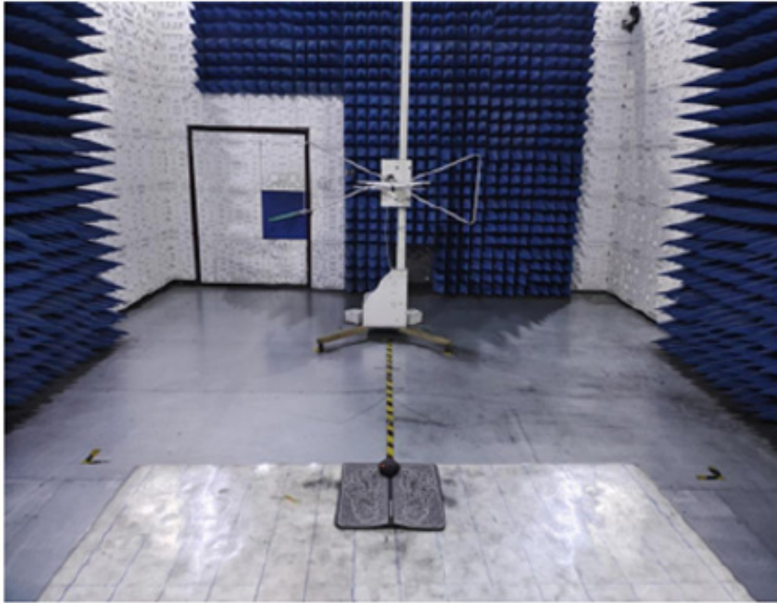
Radiated emissions at frequencies up to 1 GHz
